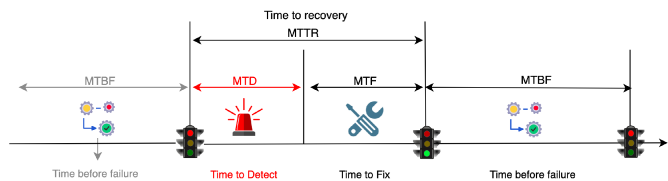
Fig. 1. Illustration on the relationship between various status
