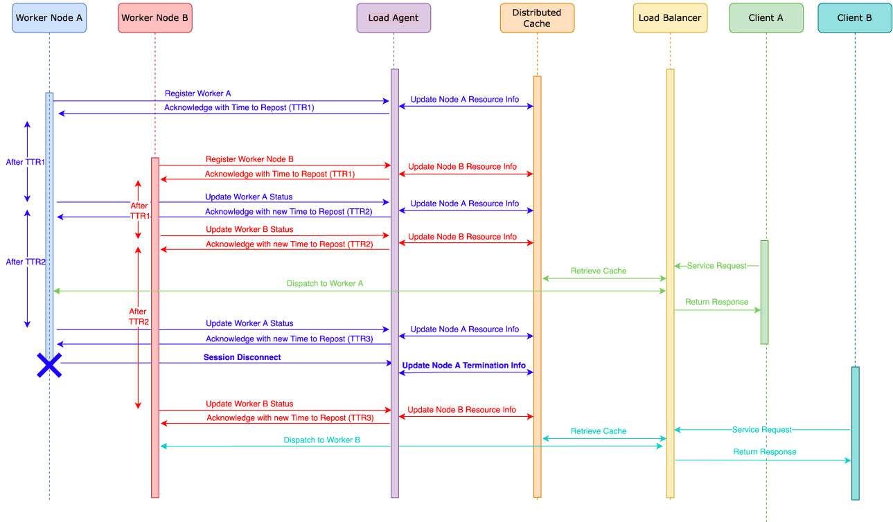
Fig. 4. Overall flow diagram to illustrate the fault event handling, recovery agent is not in scope
