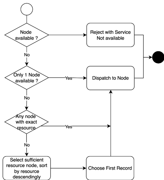
Fig. 3. Resource awareness routing algorithm (RARA)
